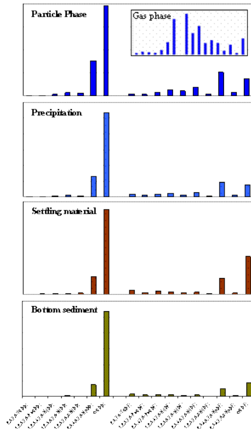
Figure 3: PCDD/F congener patterns of the deposition chain into Lake Maggiore.
