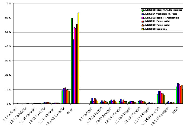
Figure 2: PCDD/F congener patterns from bottom sediments of Lake Maggiore.
